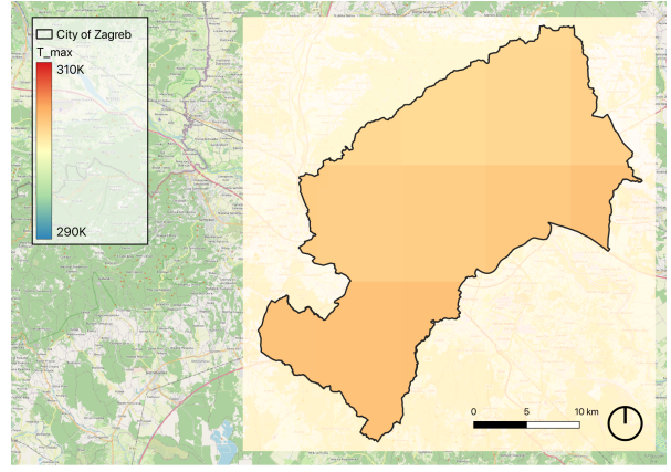
(b) Max temperature ( T_{max} ) map
